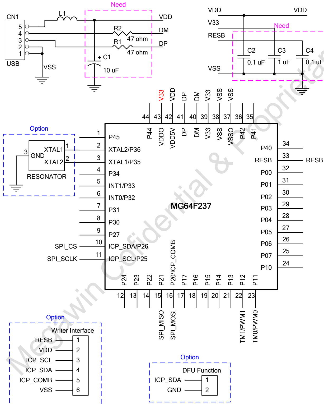
Figure 18-2 Application Circuit - Dongle
