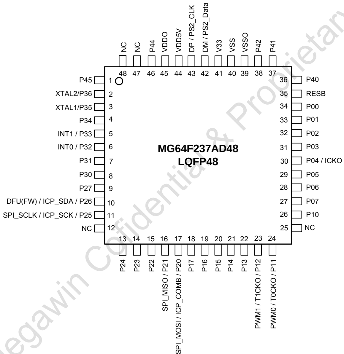
Figure 4-1 Package LQFP48
