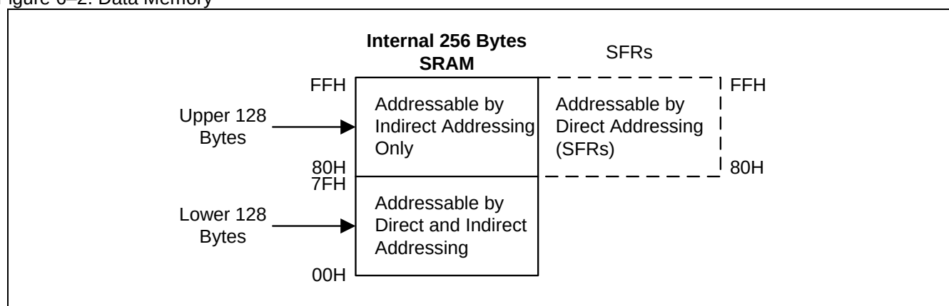
Figure 6–2. Data Memory
