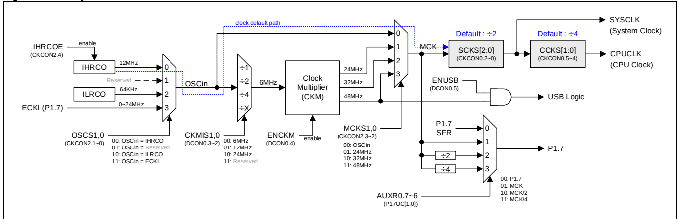
Figure 8–1. System Clock
