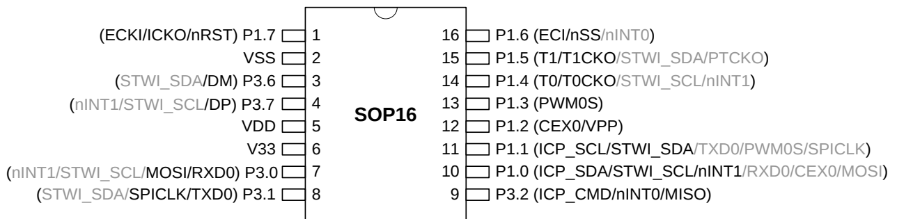
Figure 4–2. MG74PG1A08AS16 Top View
