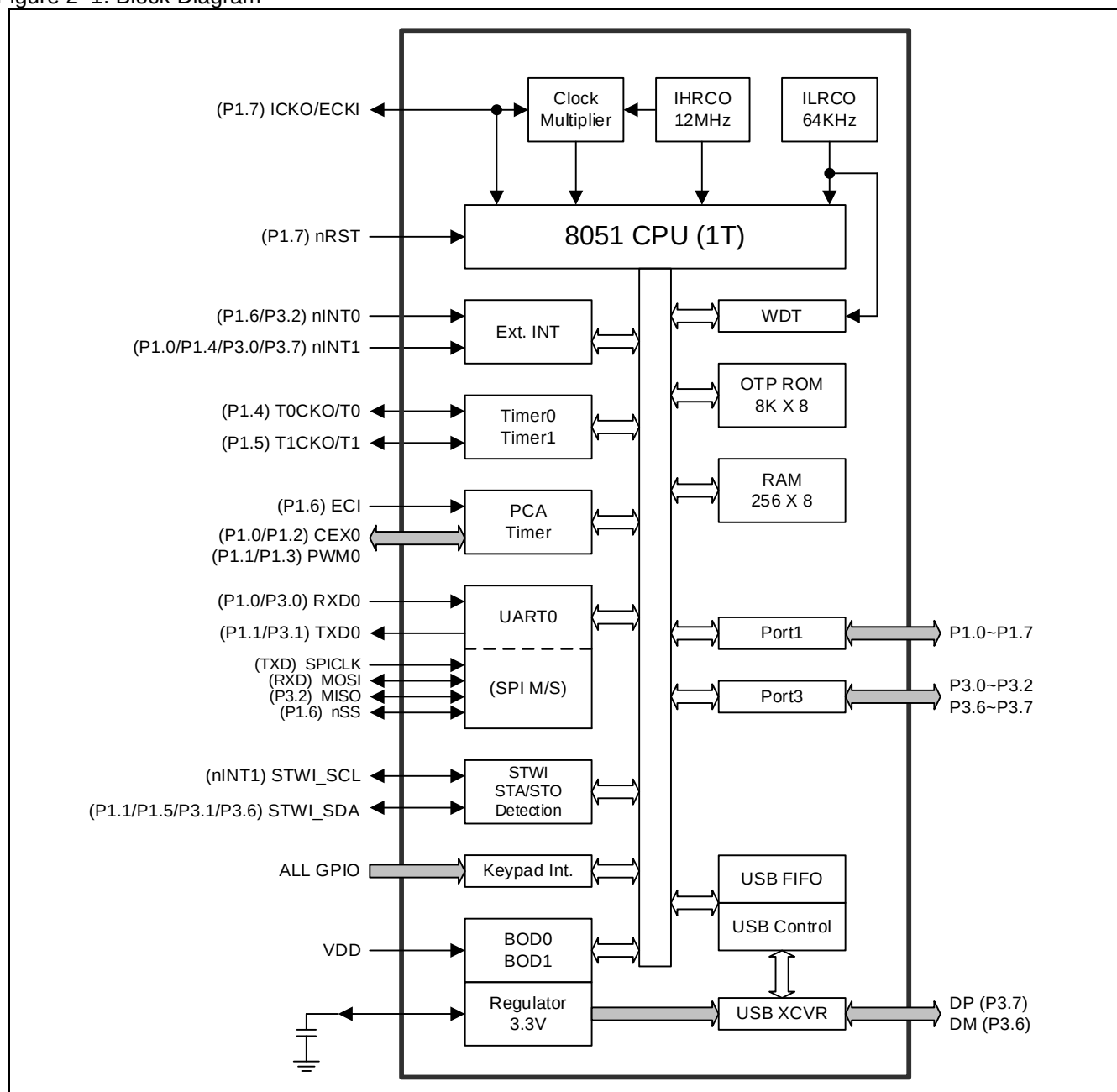
Figure 2–1. Block Diagram
