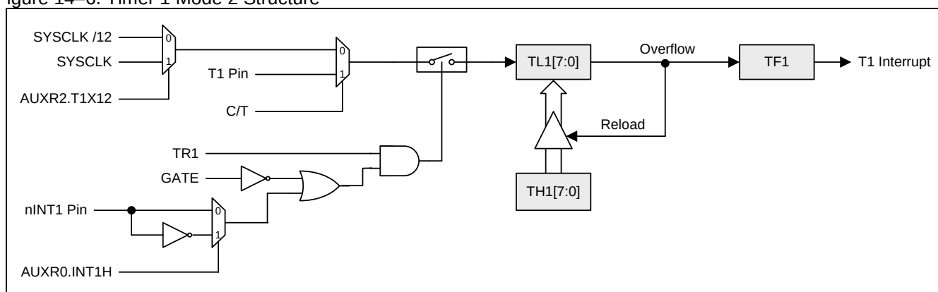
Figure 14–6. Timer 1 Mode 2 Structure
