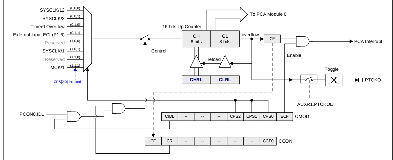
Figure 15–2. PCA Timer/Counter
