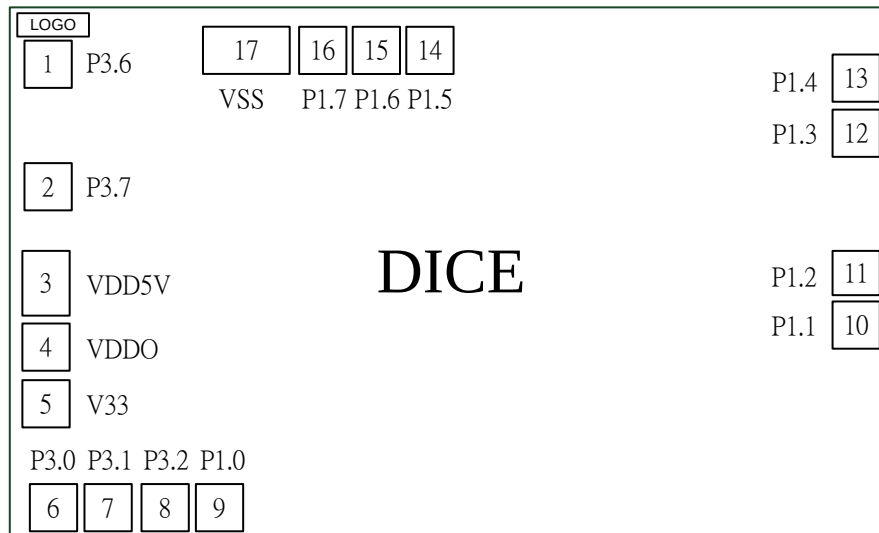
Figure 4–1. MG74PG1A08AH Top View
