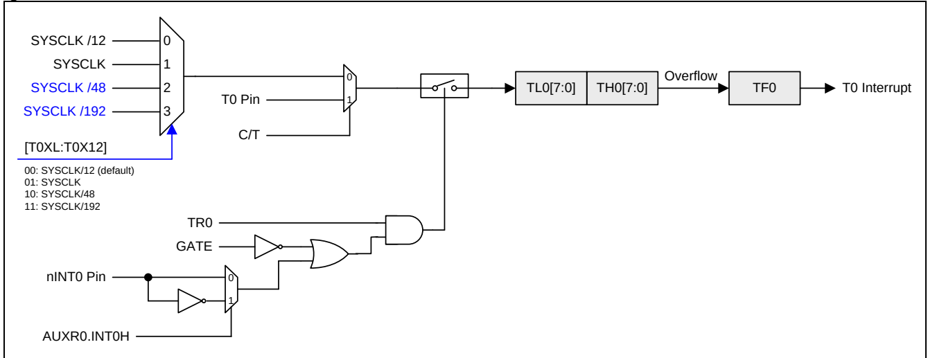
Figure 14–3. Timer 0 Mode 1 Structure
