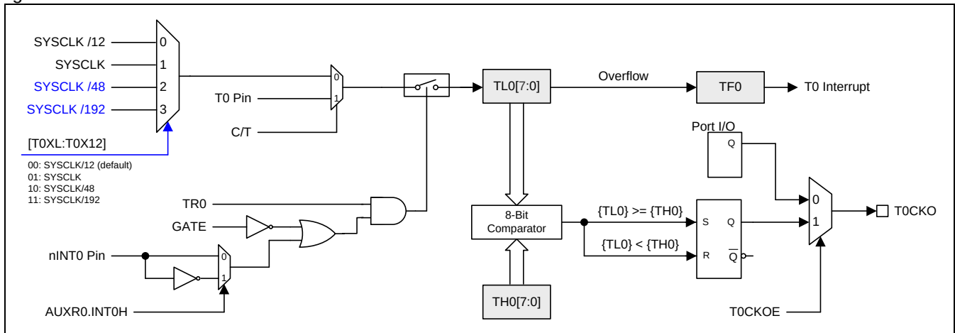
Figure 14–1. Timer 0 Mode 0 Structure
