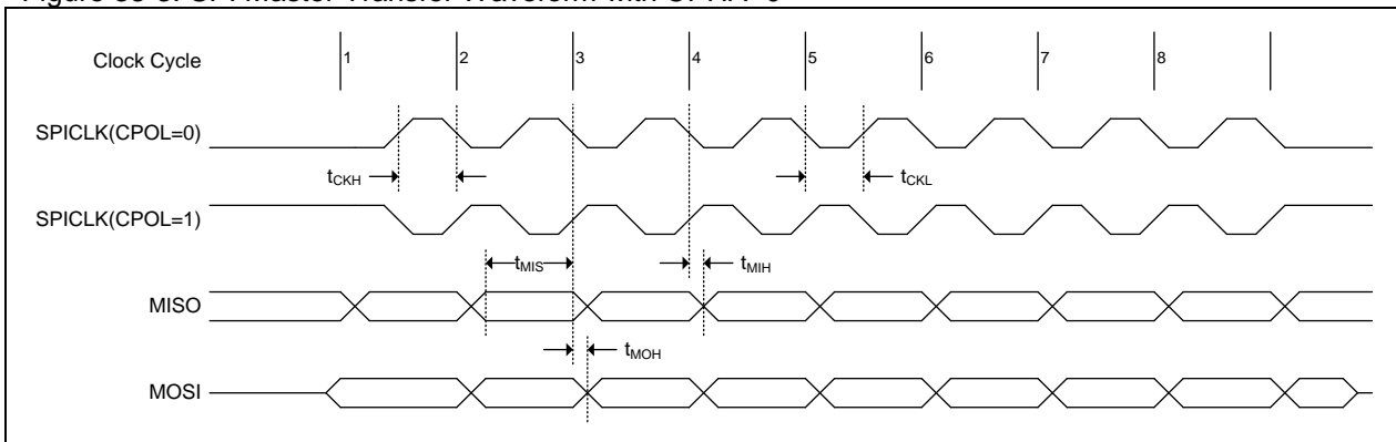
Figure 33-3. SPI Master Transfer Waveform with CPHA=0
