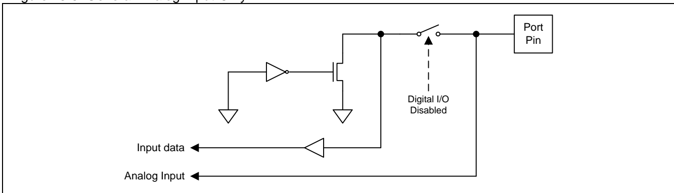
Figure 13-5. General Analog-Input-Only
