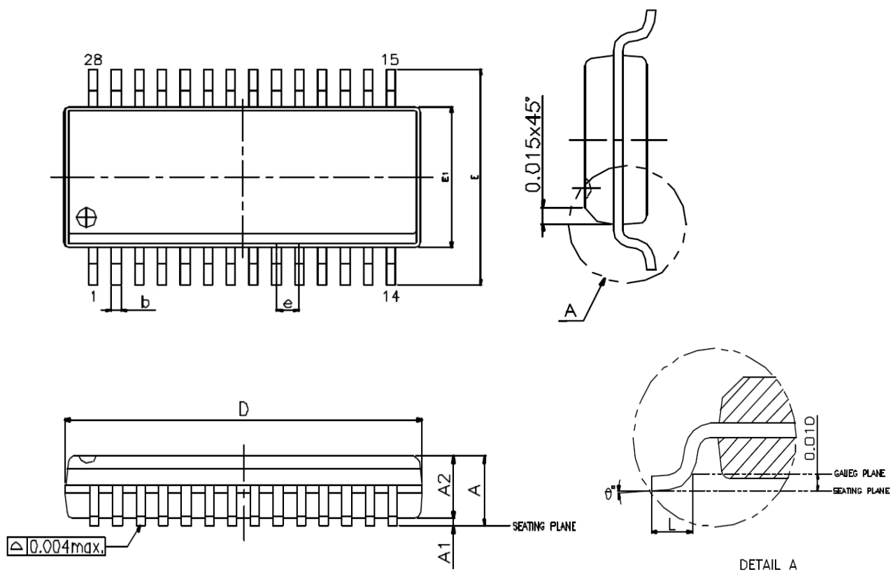
Figure 35-1. SSOP-28
