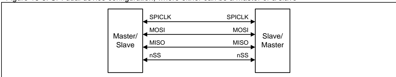
Figure 18-3. SPI dual device configuration, where either can be a master or a slave
