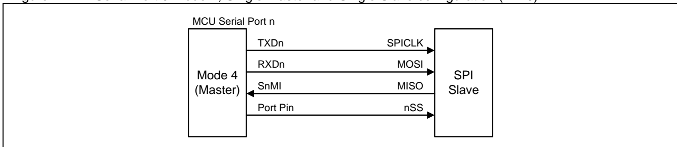
Figure 17-11. Serial Port 0 Mode 4, Single Master and Single Slave configuration (n = 0)
