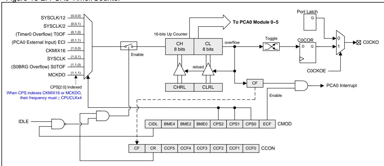
Figure 16-2. PCA0 Timer/Counter
