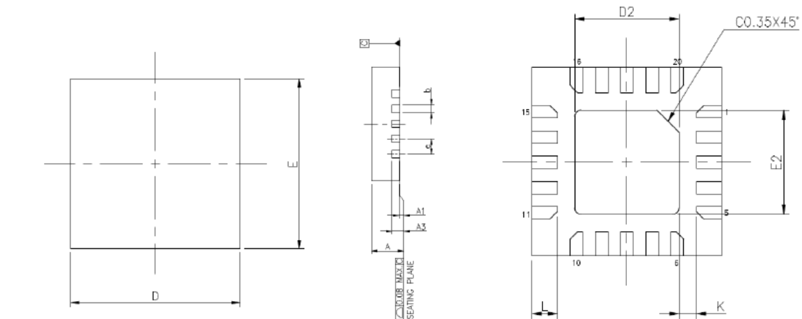
QFN 20P(3x3mm) package dimension
