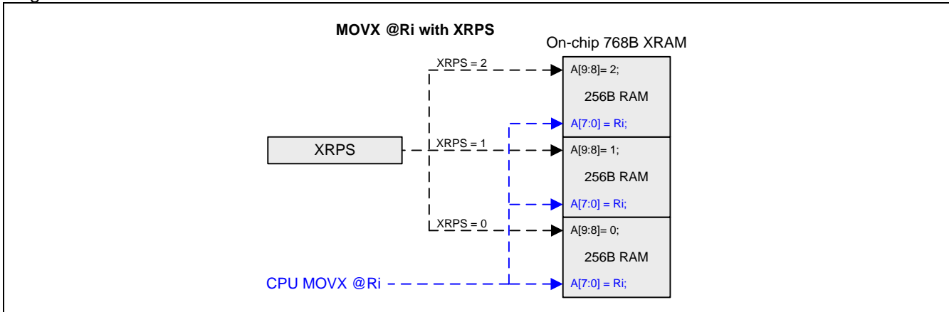
Figure 7-2. XRPS Structure
