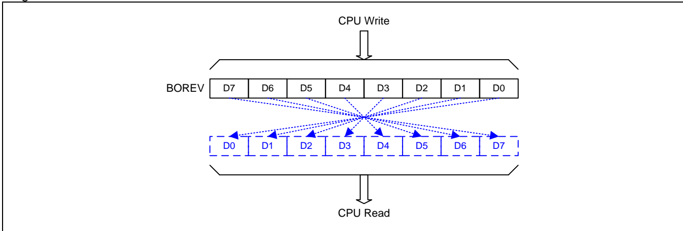
Figure 23–2. BOREV structure
