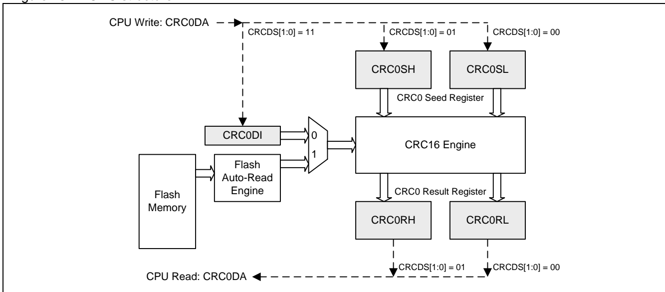
Figure 23–1. CRC structure
