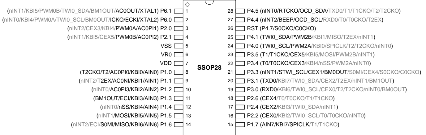
Figure 4-1. SSOP28 Top View
