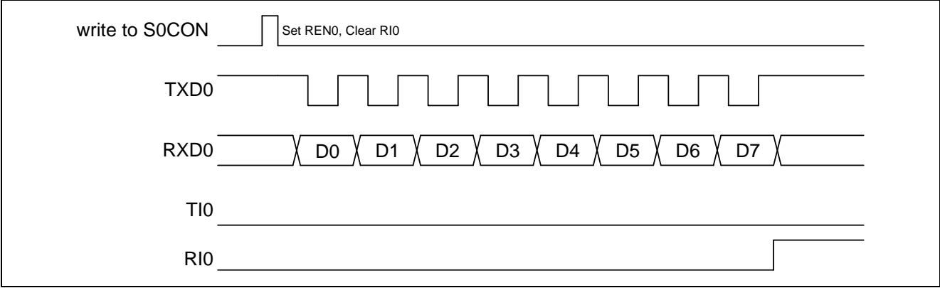
Figure 17-5. Mode 0 Reception Waveform
