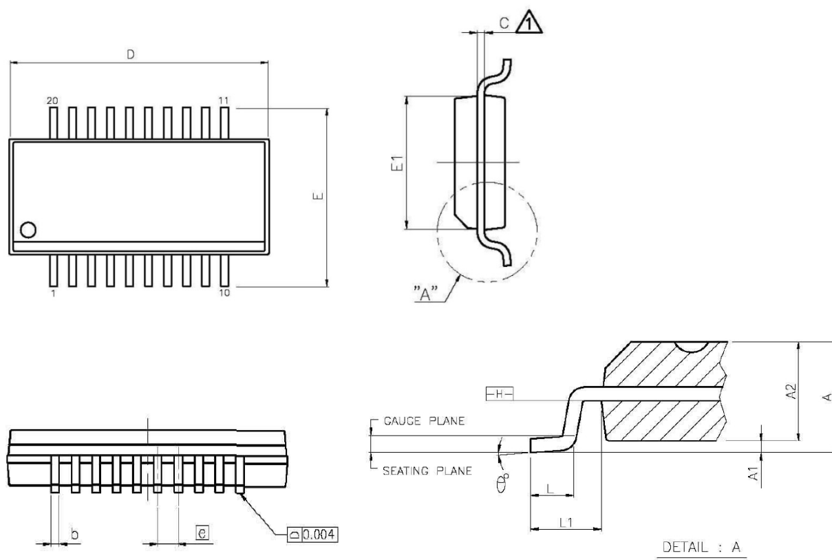
Figure 35-2. SSOP20 (150 mil) Package dimension
