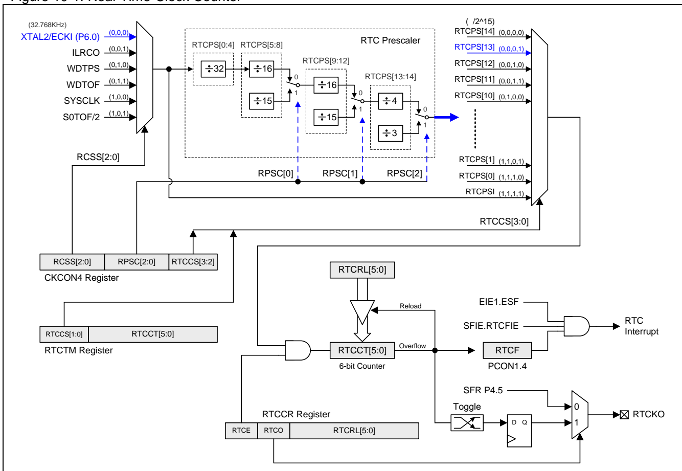
Figure 10-1. Real-Time-Clock Counter
