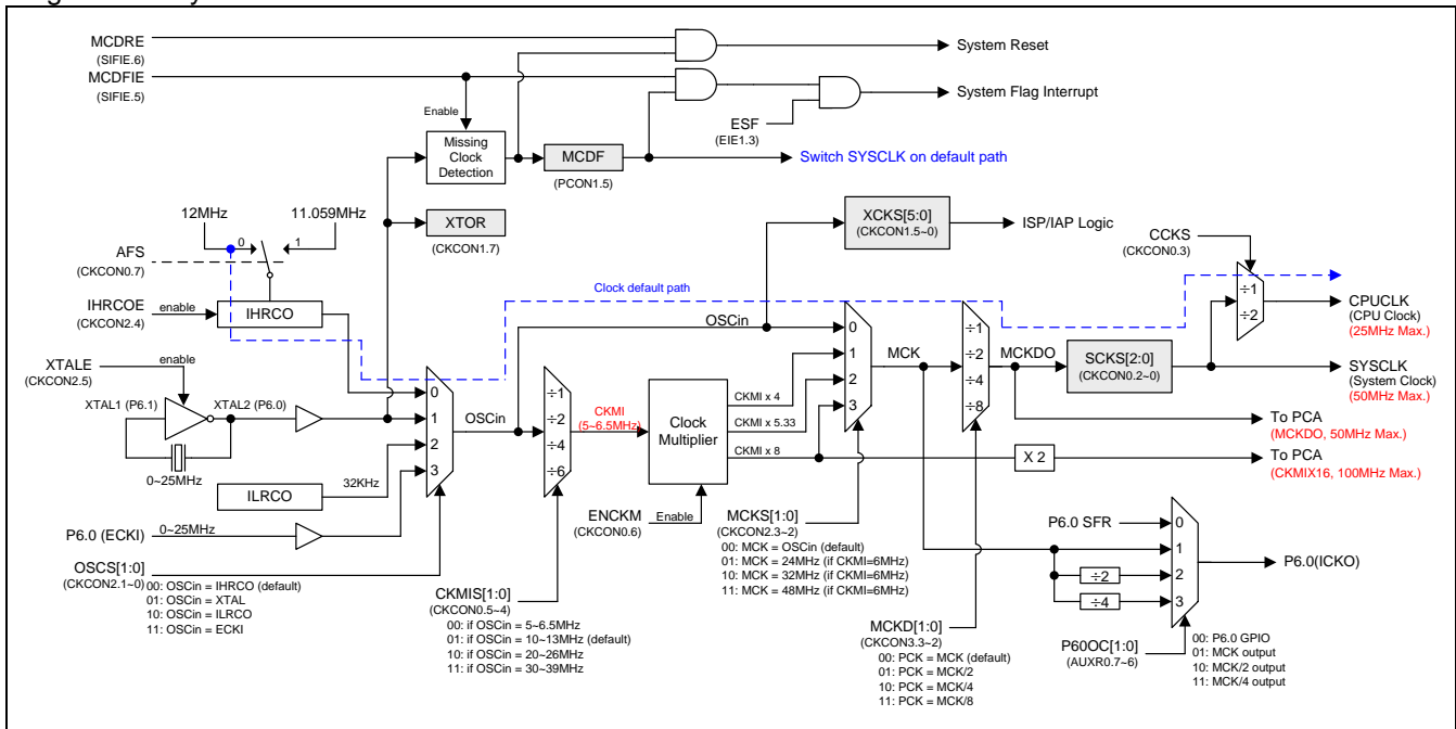
Figure 8-1. System Clock
