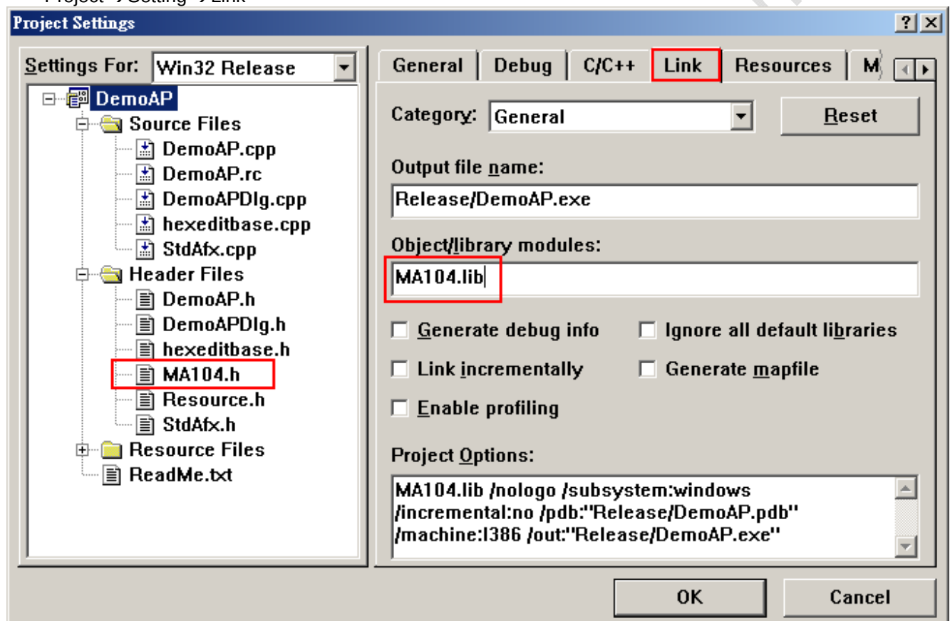
Figure 8-2 Link MA104.DLL
