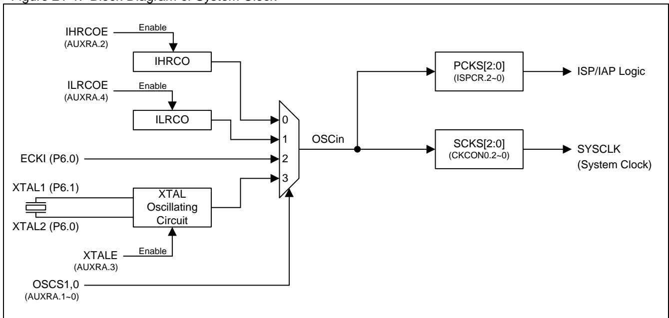
Figure 21-1. Block Diagram of System Clock
