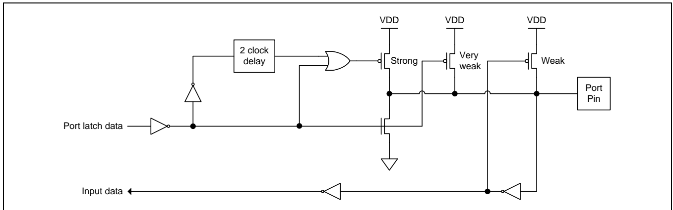
Figure 9-1 Quasi-Bidirectional I/O
