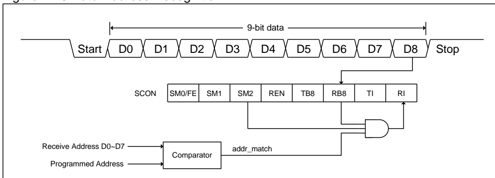
Figure 12-9 Auto-Address Recognition
