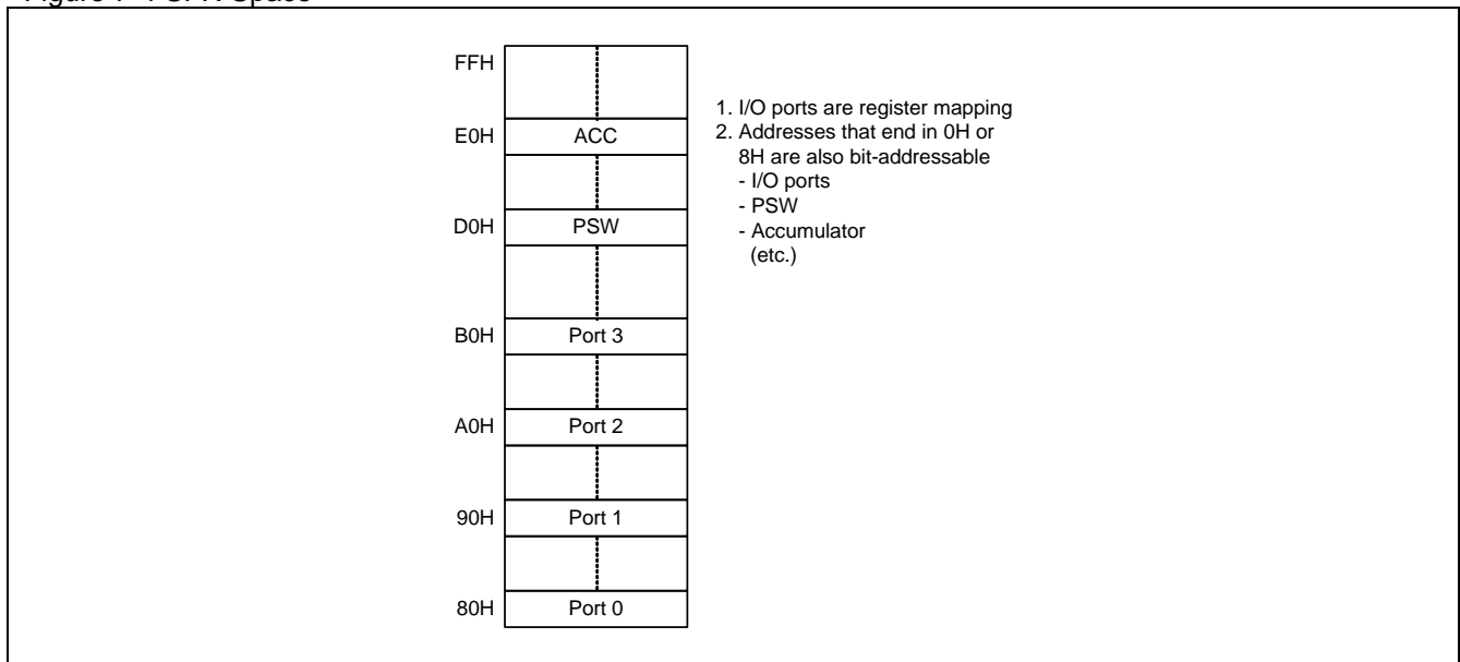
Figure 7-4 SFR Space
