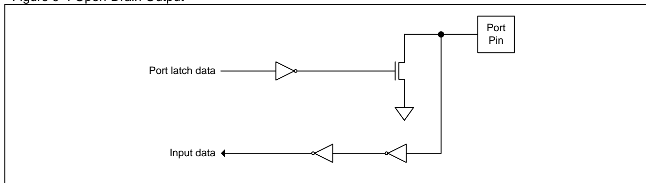
Figure 9-4 Open-Drain Output
