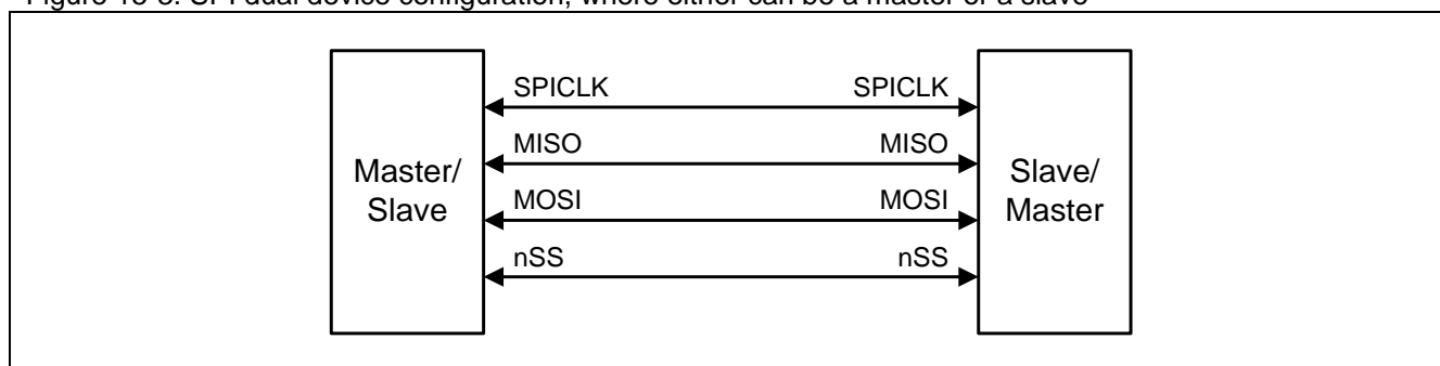
Figure 15-3. SPI dual device configuration, where either can be a master or a slave
