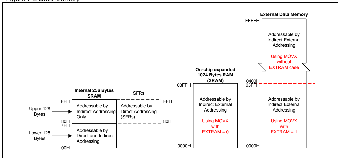
Figure 7-2 Data Memory
