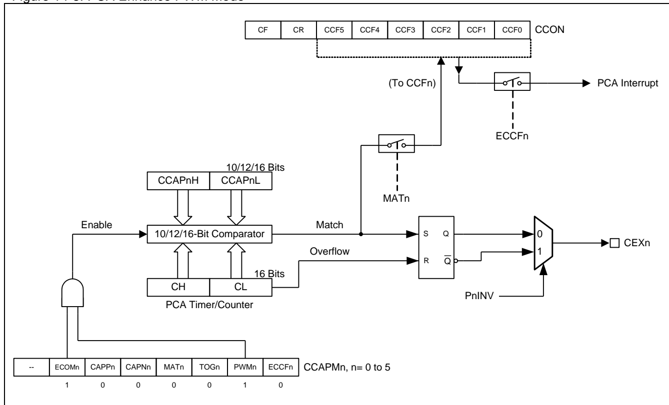
Figure 14-8. PCA Enhance PWM Mode
