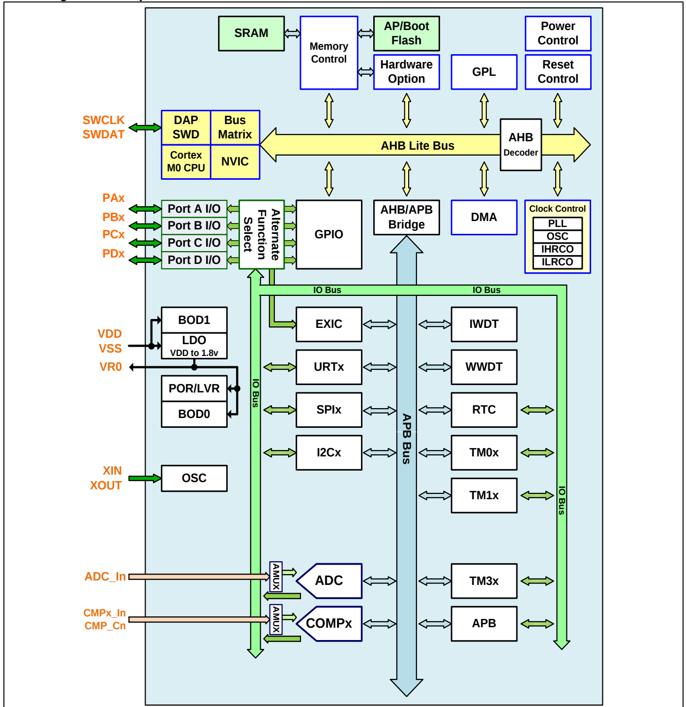
Figure 3-2. Chip Main Block
