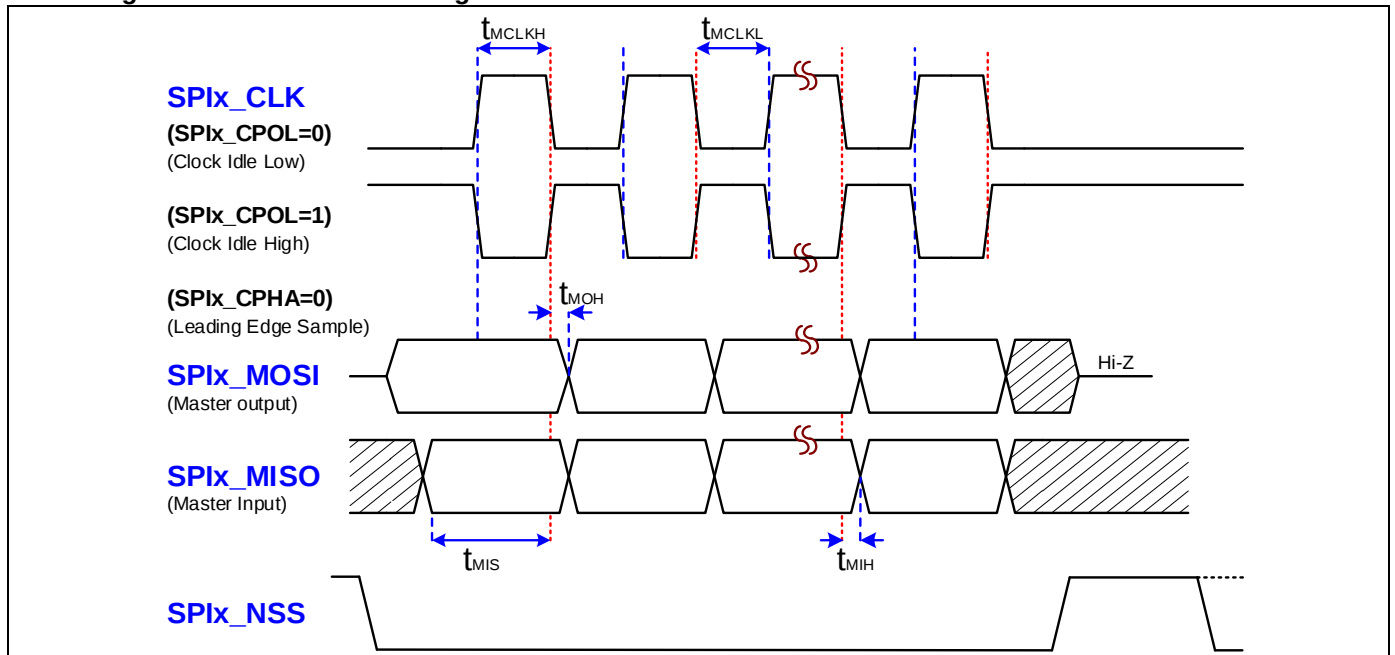
Figure 8-2. SPI Master Timing Waveform
