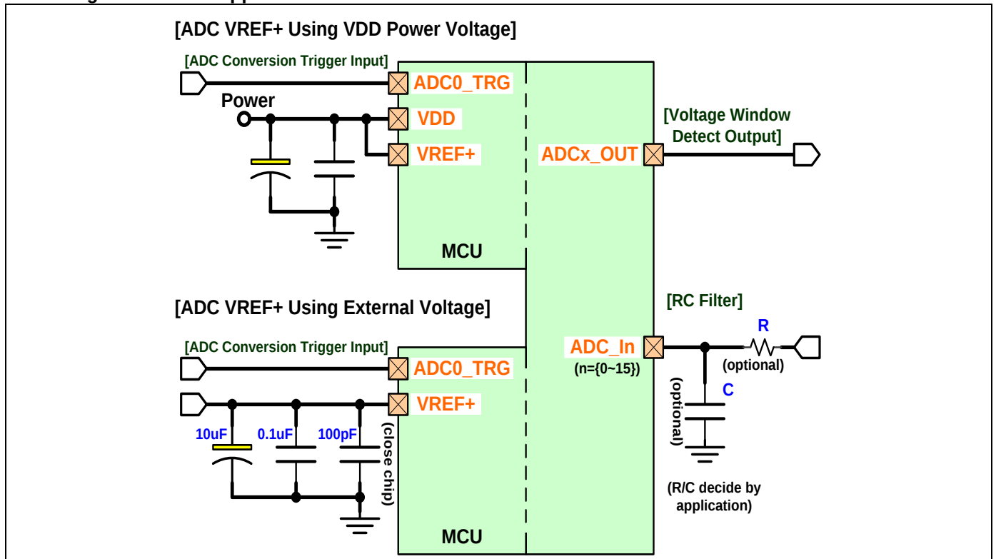
Figure 7-4. ADC Application Circuit
