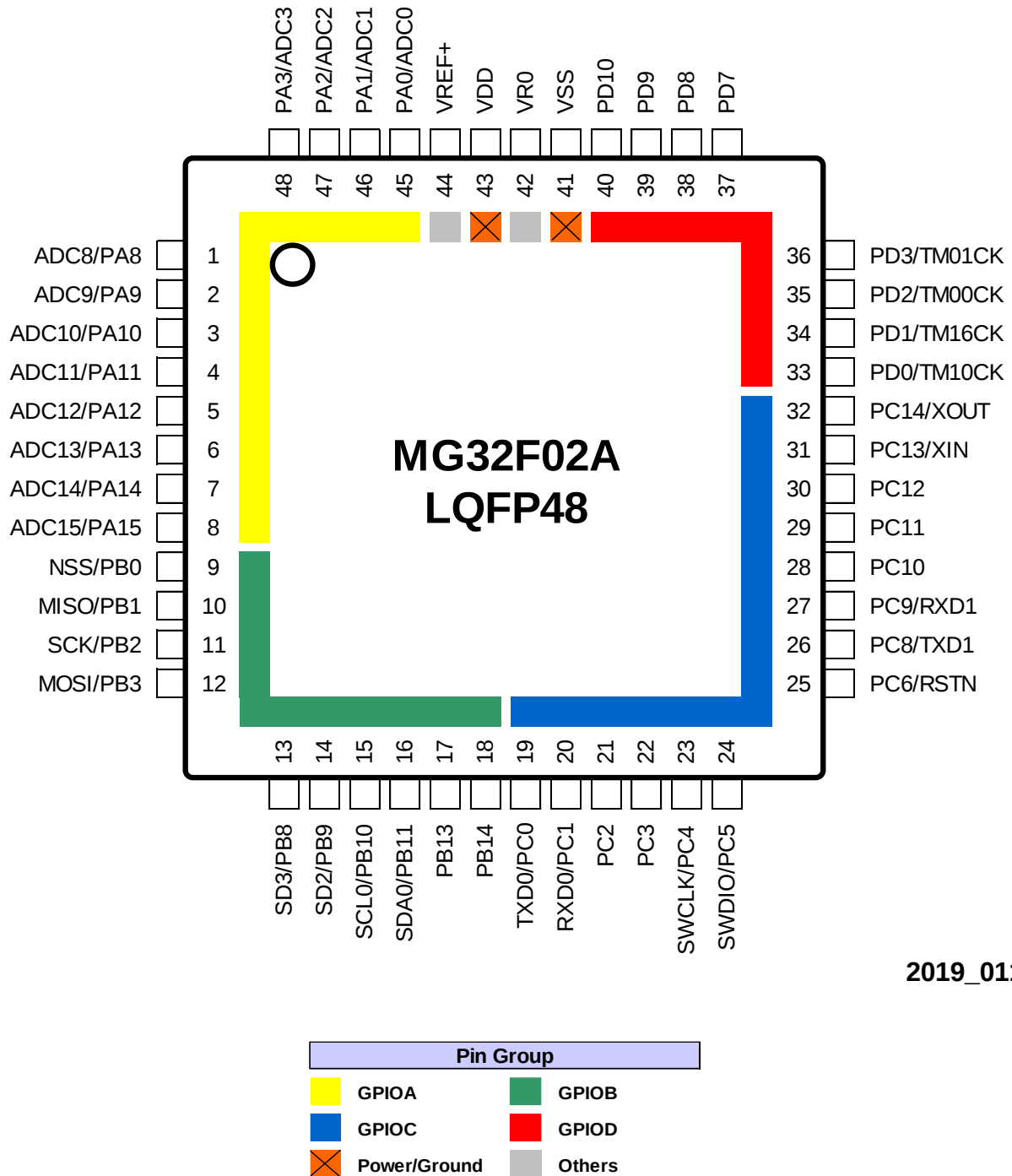
Figure 4-1. LQFP48 Package Pinout
