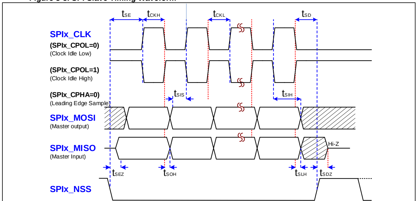
Figure 8-3. SPI Slave Timing Waveform
