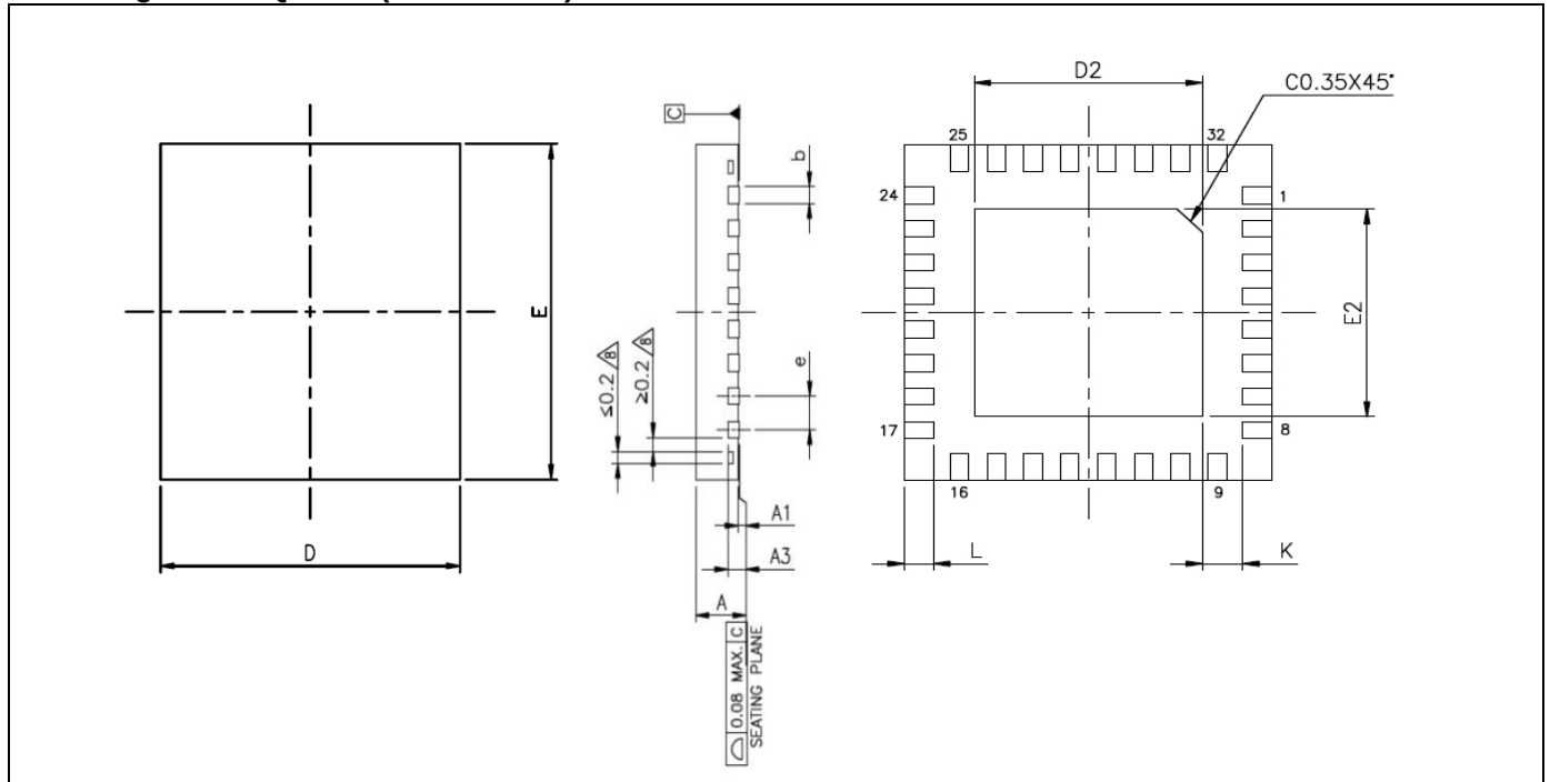
Figure 9-2. QFN-32 (5mm X 5mm) ~ AY32
