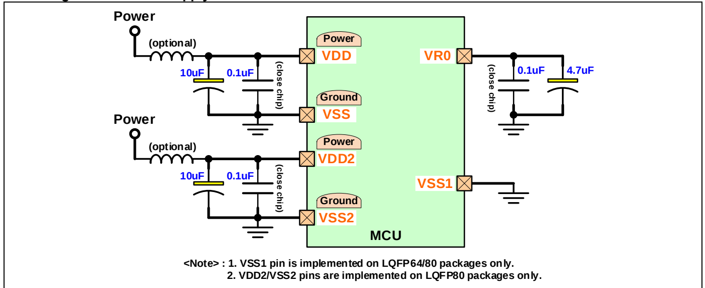
Figure 7-1. Power Supply Circuit
