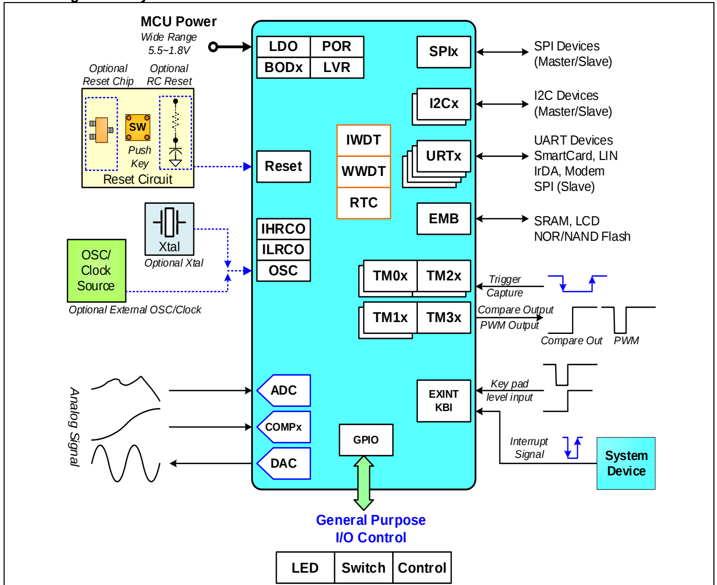
Figure 3-1. System Function Block
