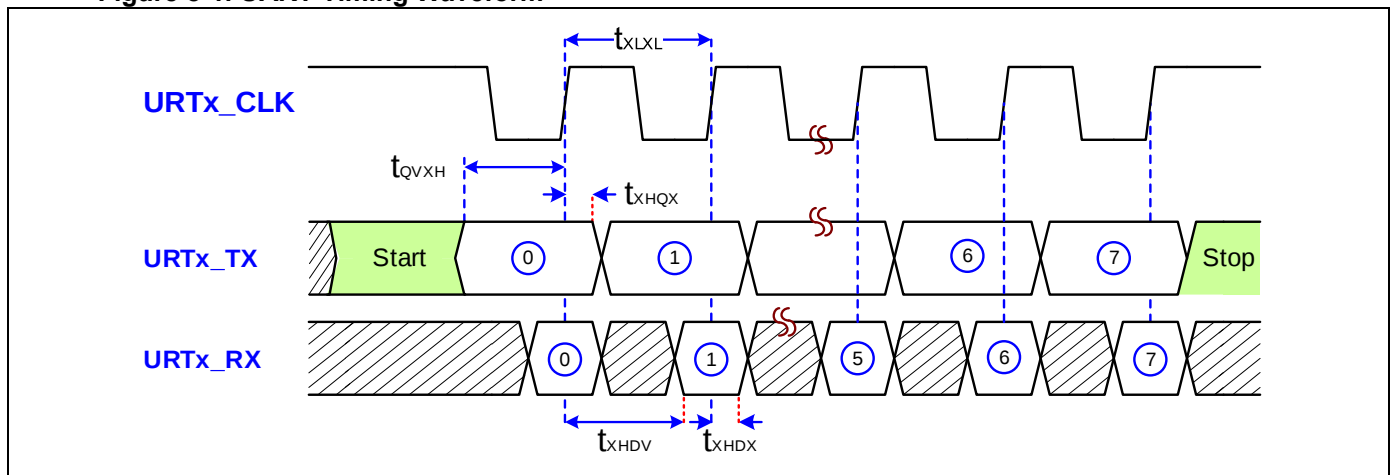
Figure 8-1. UART Timing Waveform
