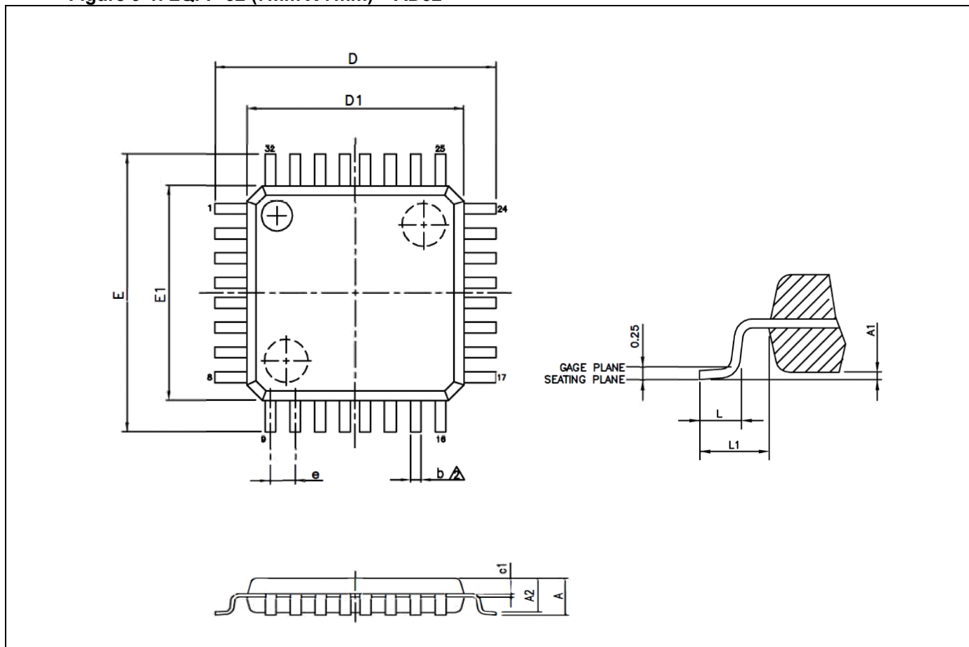
Figure 9-1. LQFP-32 (7mm X 7mm) ~ AD32
