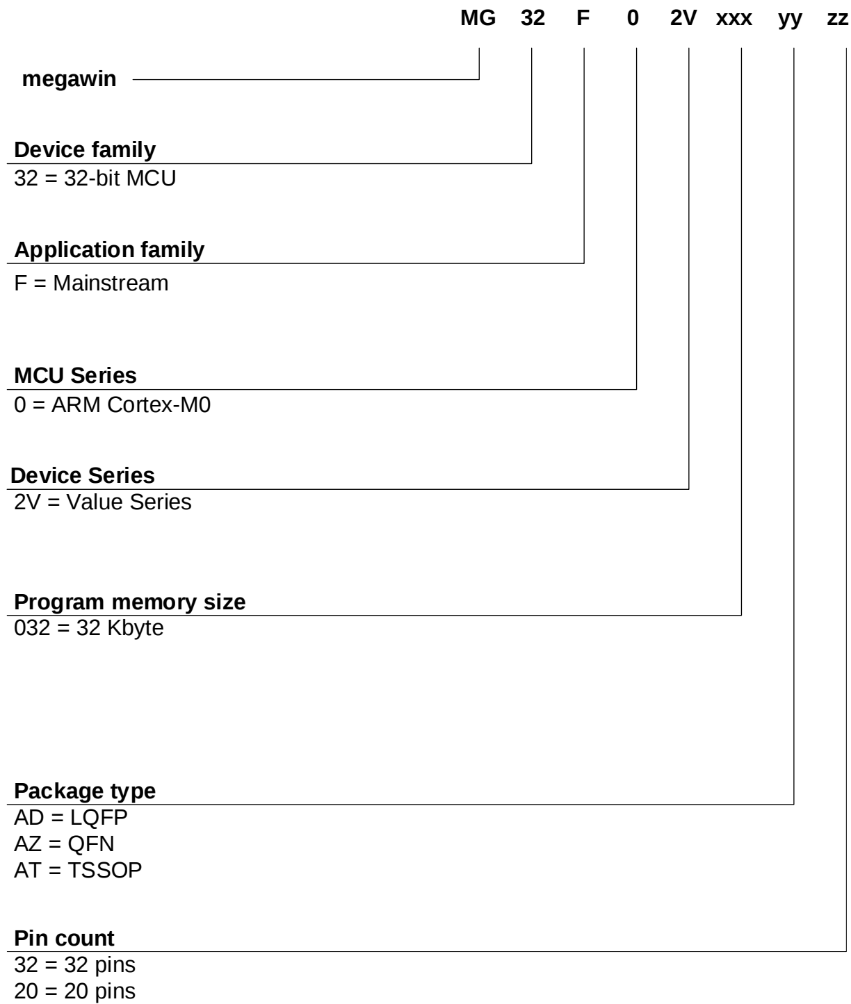
Figure 2-1. Part Numbering
