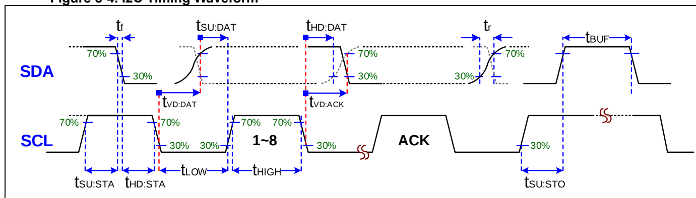
Figure 8-4. I2C Timing Waveform
